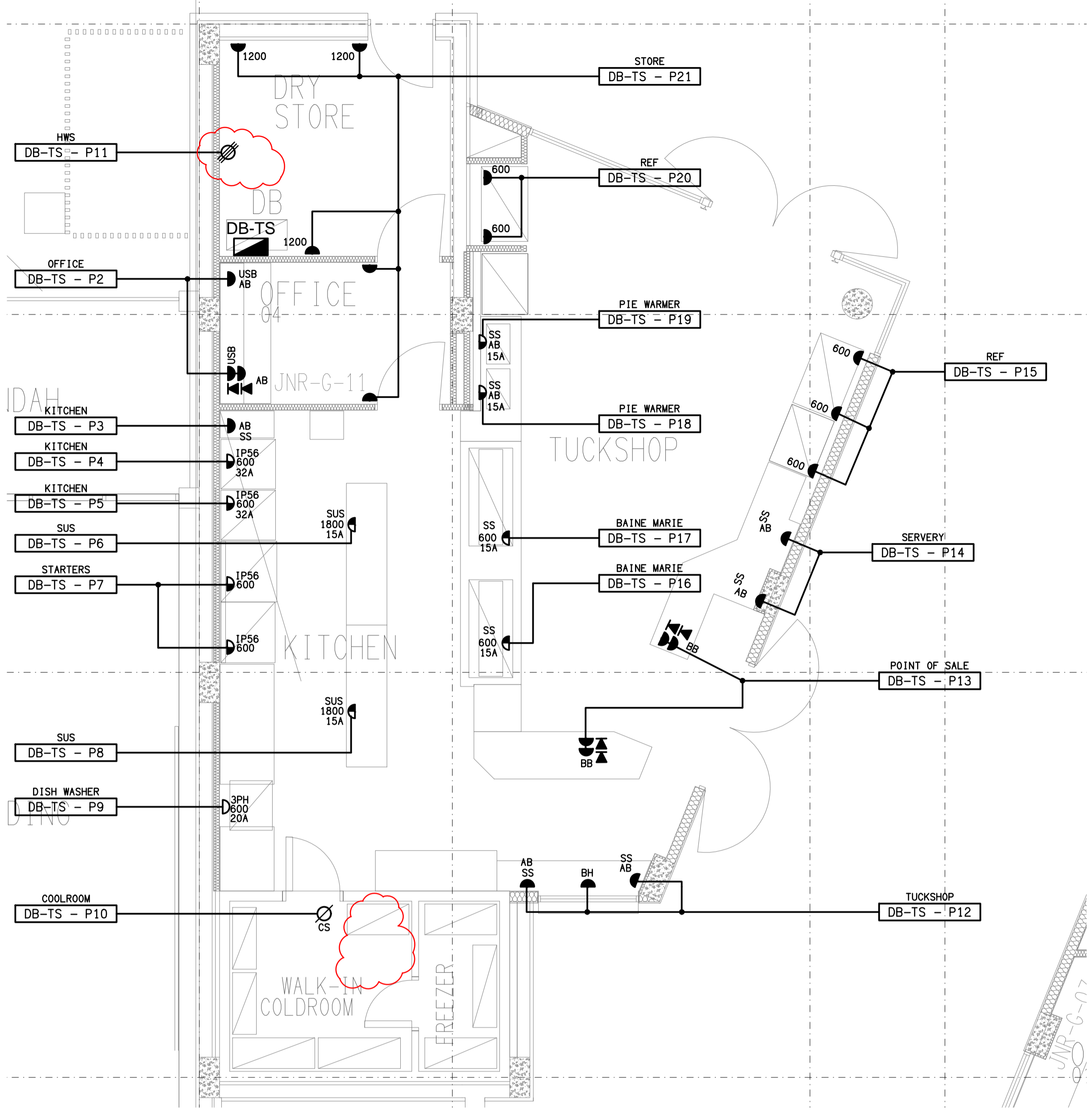
TUCKSHOP GROUND LEVEL FLOOR PLAN SCALE 1:50
